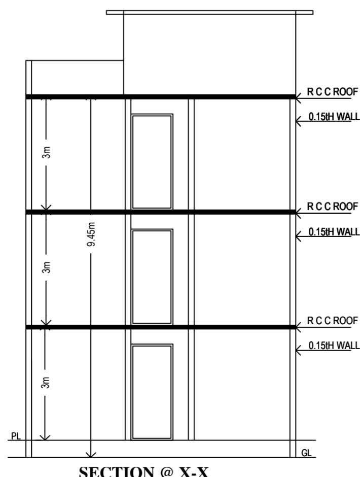
SECTION @ X-X
